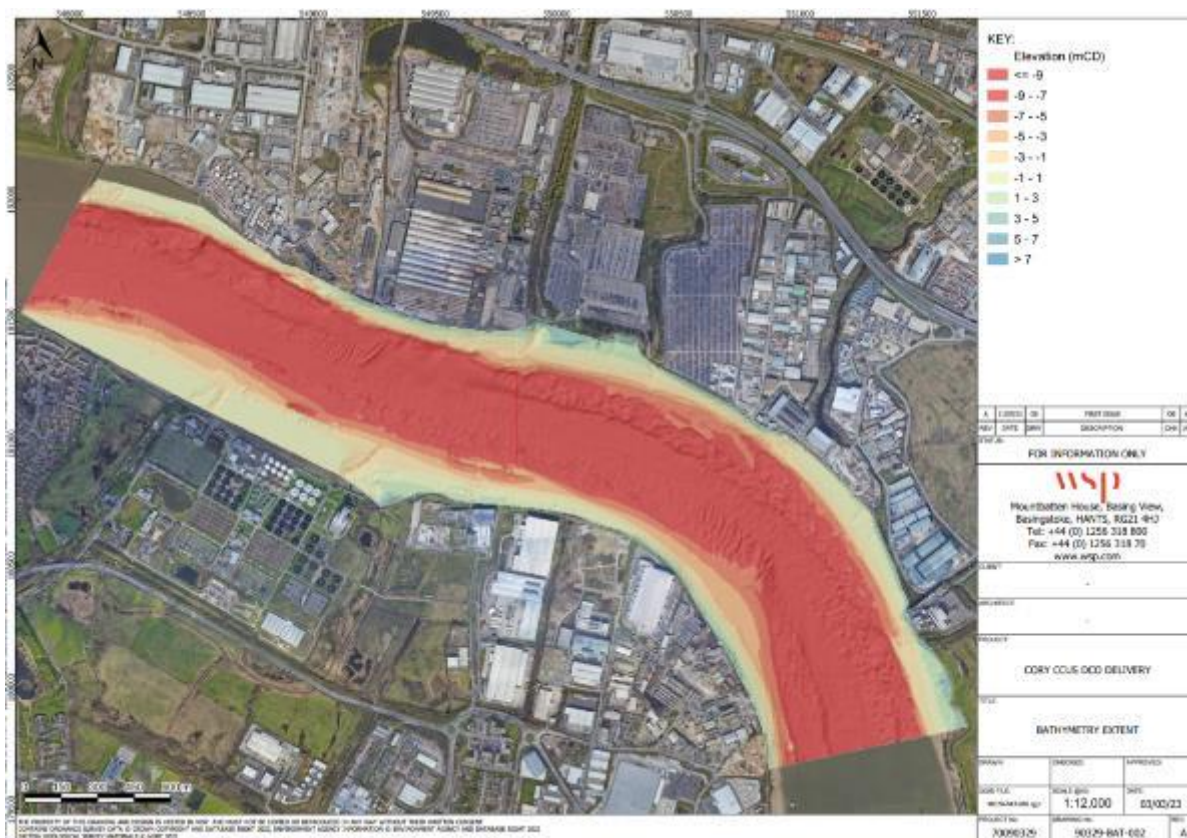
Figure 10: Bathymetric Survey (mCD)
