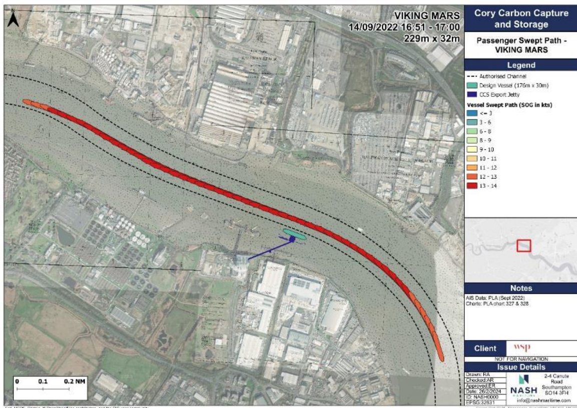
Figure 40: Swept Path, Passenger Vessel Outbound ( Viking Mars )
